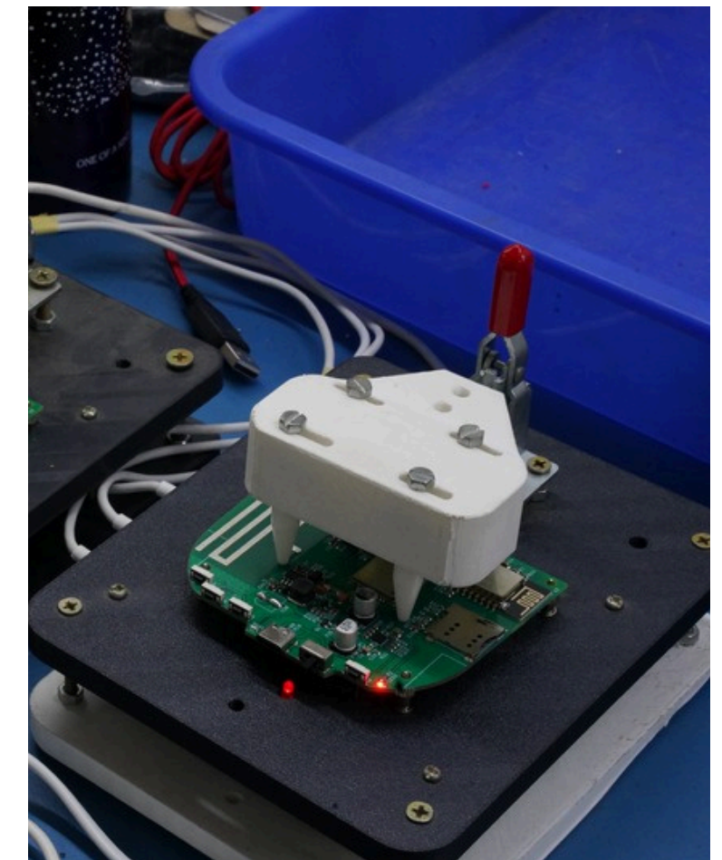
PCB Programming
